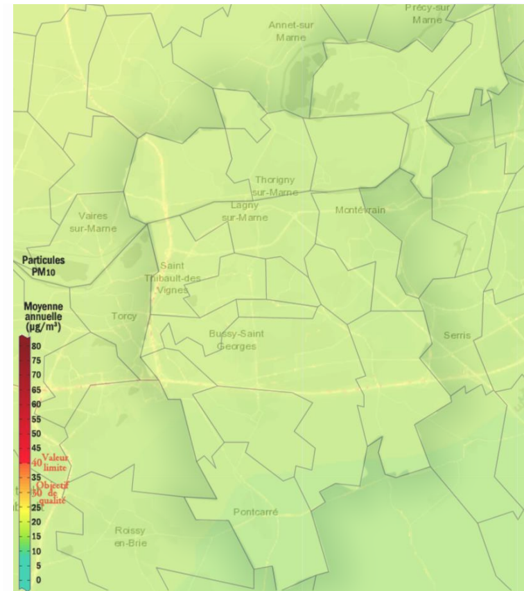
PM 10 – 2019 - AIRPARIF
